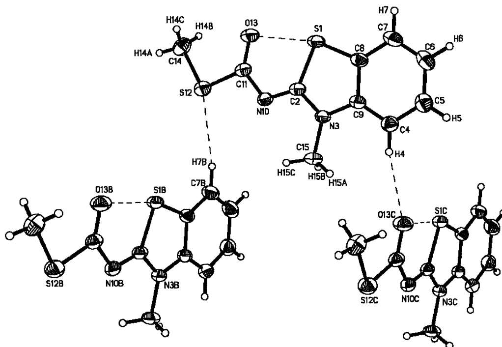
Figure 5. Molecular structure of compound 7 showing intra- and intermolecular interactions
