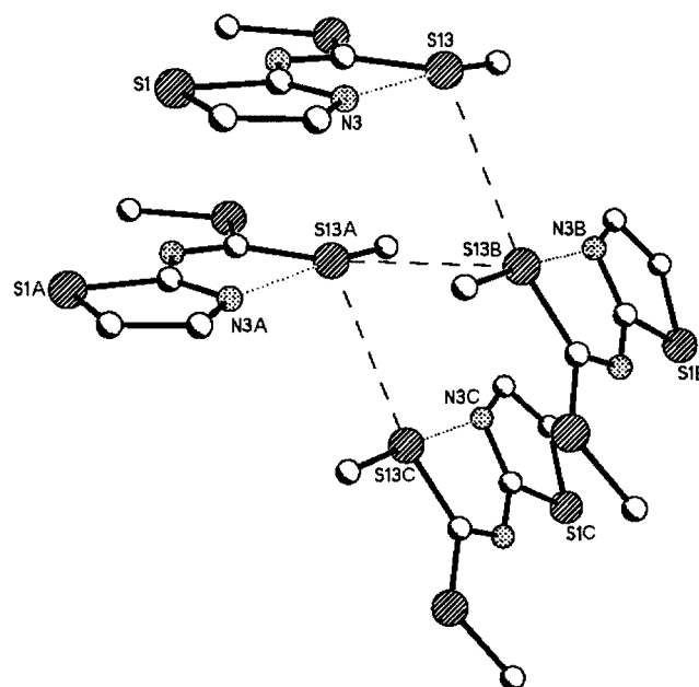
Figure 3. Molecular structure of compound 4; intra- and intermolecular interactions are shown
