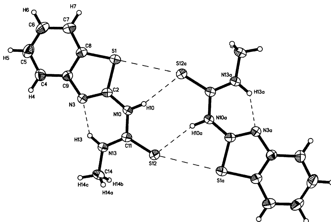
Figure 7. Molecular structure of compound 9 and intra- and intermolecular interactions
