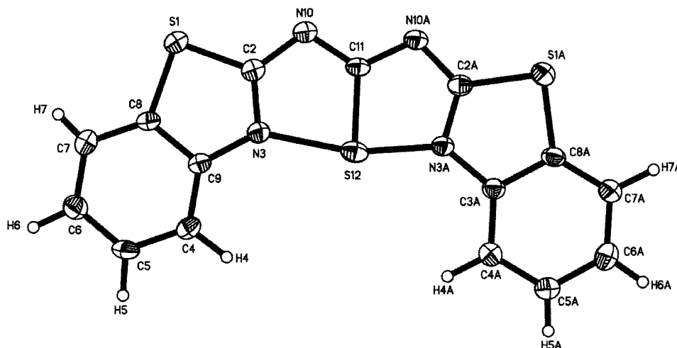
Figure 10. Molecular structure of compound 16
