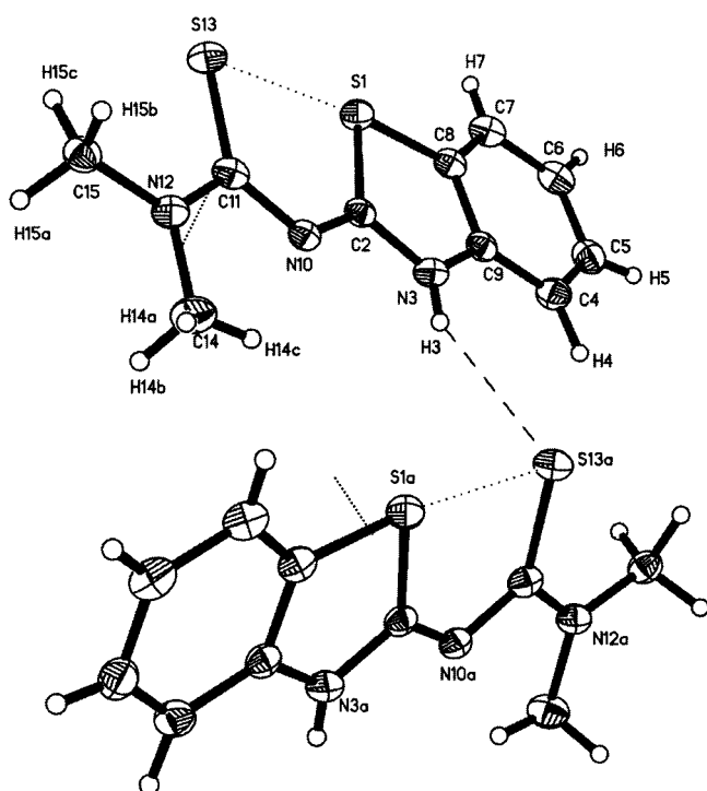
Figure 6. Molecular structure of compound 8 and intra- and intermolecular hydrogen bonds
