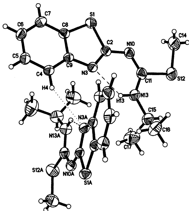
Figure 9. Molecular structure of compound 13
