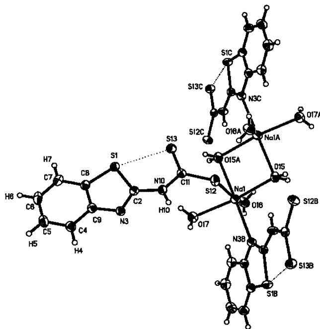
Figure 1. Molecular structure of compound 3-Na
