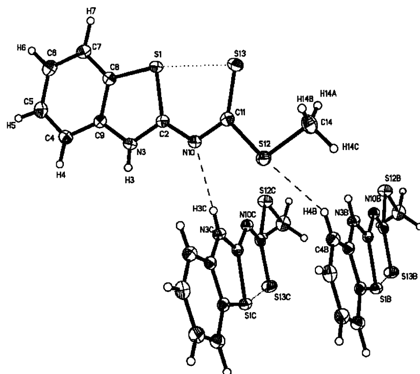
Figure 4. Molecular structure of compound 5; intra- and intermolecular interactions are shown
