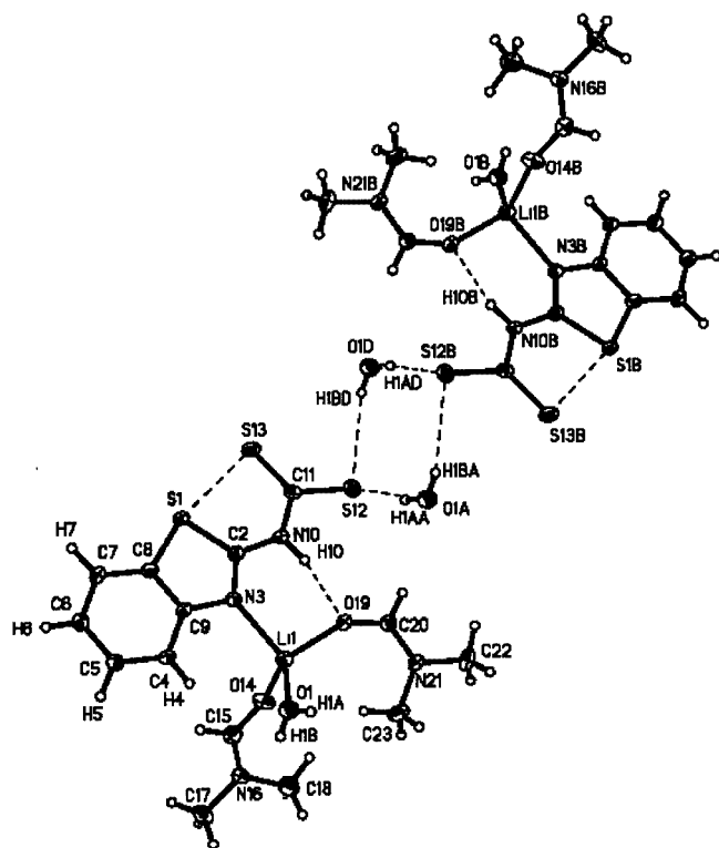
Figure 2. Molecular structure of compound 3-Li
