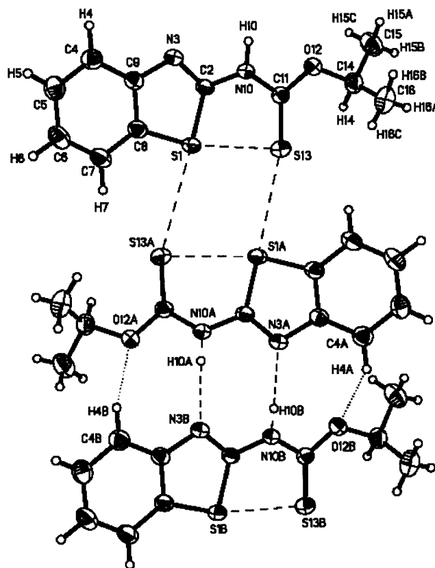
Figure 8. Molecular structure of compound 11 showing intra- and intermolecular interactions
